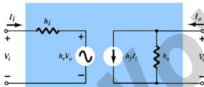
Hybrid Equivalent Circuit
