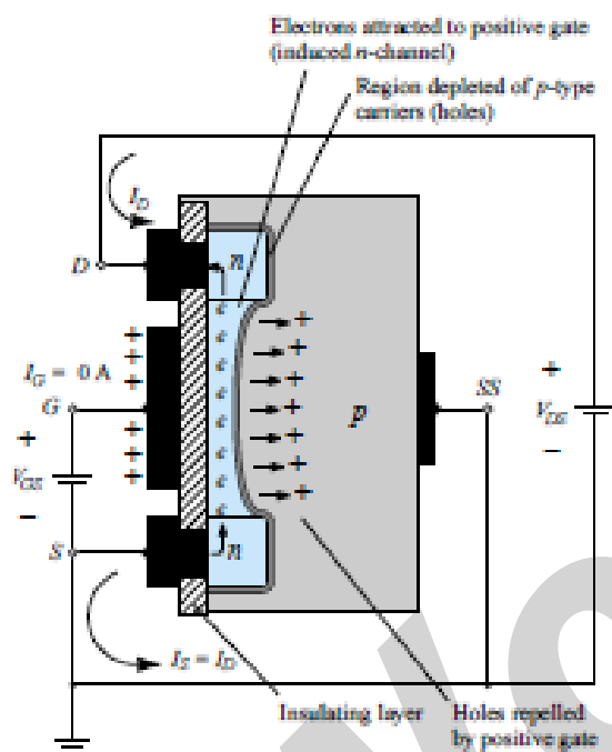
Fig 2. Channel formation
