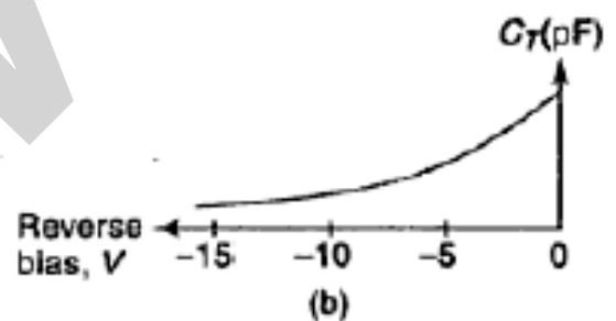
(a) Circuit symbol of varactor diode (b) Characteristics of varactor diode
