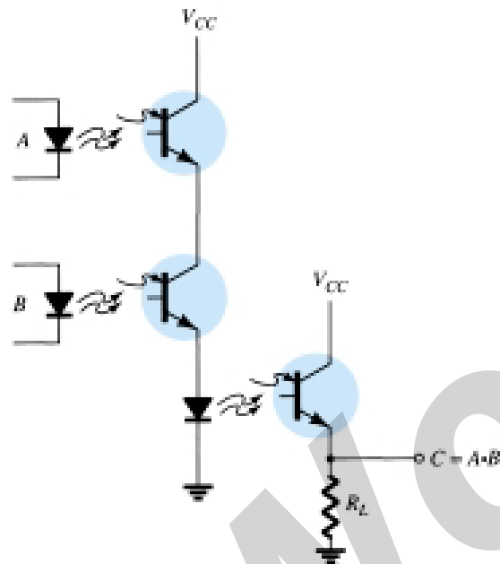
High isolation AND gate employing phototransistor and LED
