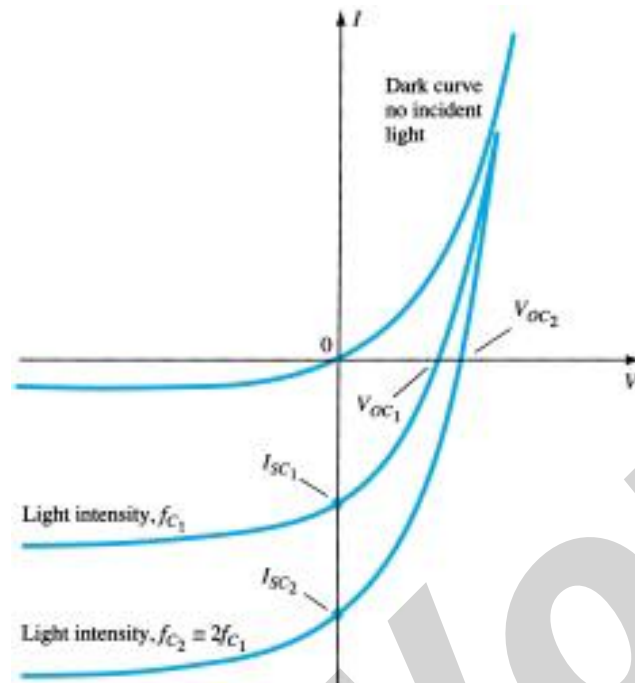
Fig 2. V-I curve for solar cell
