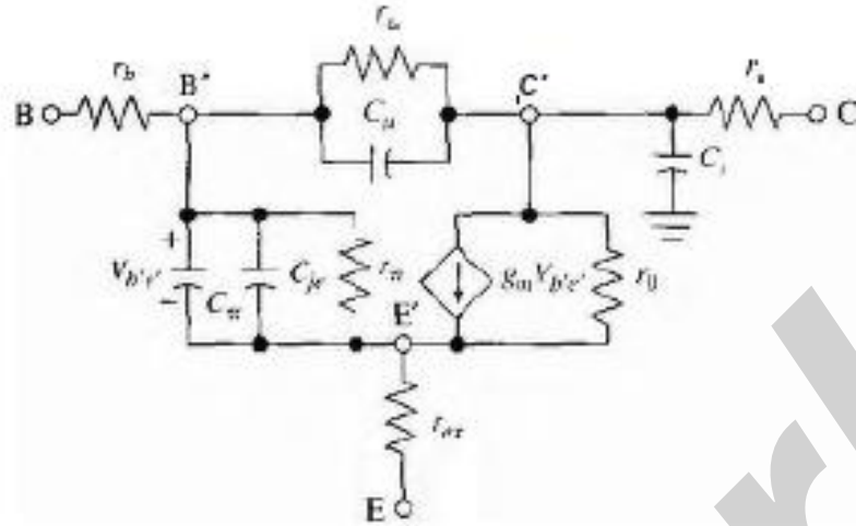
Figure 3 Hybrid-pi equivalent circuit.
